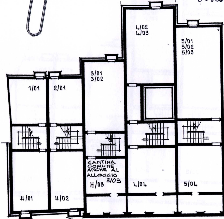
PIANO CANTINATO
